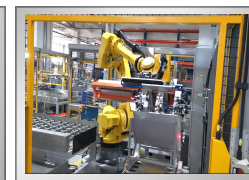
铝饰板全自动分离装备 Aluminum trim plate automatic separation machine
