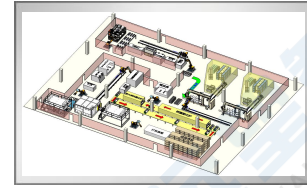
氢瓶全自动装配检测线 Hydrogen bottle automatic assembly line test line
