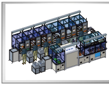
多通水阀自动装配生产线 Multi water valve automatic assembly line
