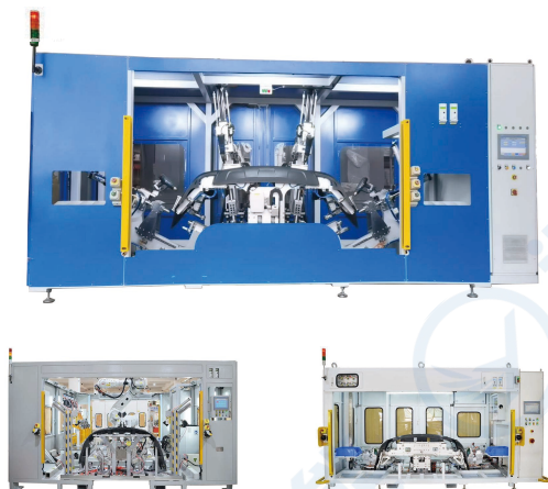
保险杠冲孔焊接一体机 Punching and welding machine for bumper
